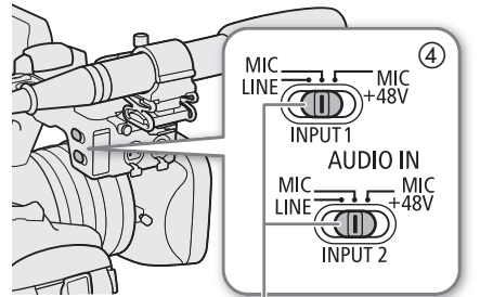
INPUT 1 / INPUT 2 switches (audio source selection)
