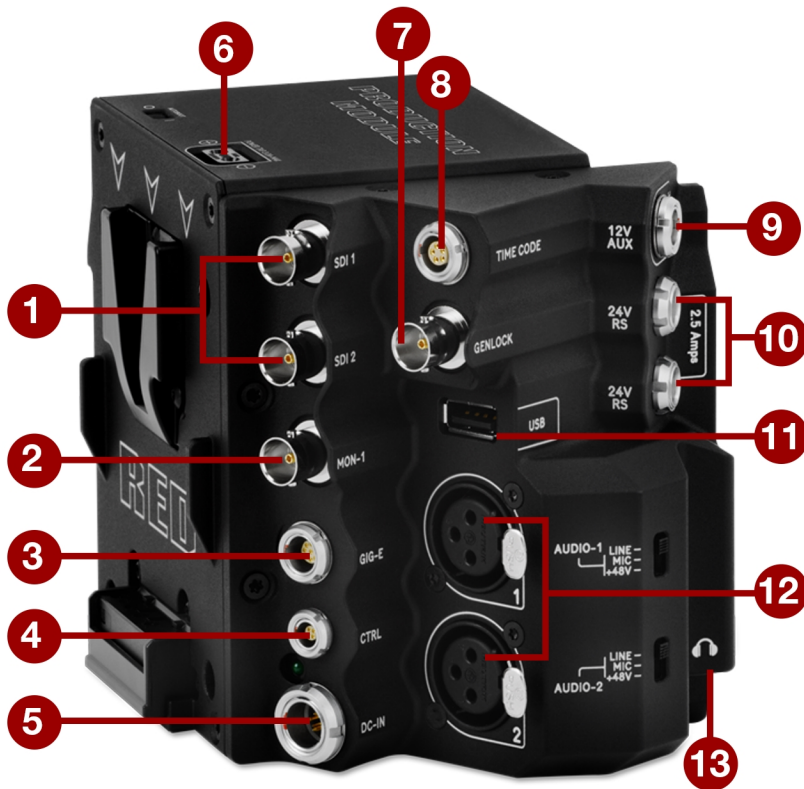
Figure: DSMC2 Production Module (V-Lock)
